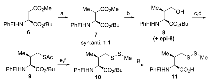
Scheme 3. Reagents and conditions: a) KHMDS, MeI, THF, -78^\circ\text{C} , 3 h, 97%; b) DIBAL-H, THF, -35^\circ\text{C} , 1 h, 83% (combined yield for 8 and epi-8 ); c) MsCl, \text{Et}_3\text{N} , \text{CH}_2\text{Cl}_2 , 0^\circ\text{C} , 1 h; d) AcSH, DBU, DMF, RT, 16 h, 73% in 2 steps; e) 1 N NaOH, MeOH, 0^\circ\text{C} , 10 min; f) MMTS, \text{Et}_3\text{N} , \text{CH}_2\text{Cl}_2 , RT, 30 min, 86% in 2 steps; g) HCl in EtOAc, RT, 82%. KHMDS = potassium 1,1,1,3,3,3-hexamethylidisilazane; DIBAL-H = diisobutylaluminum hydride; Ms = methylsulfonyl; Ac = acetyl; DBU = 1,8-diazabicyclo[5.4.0]undec-7-ene; MMTS = S-methyl methane-thiosulfonate.
